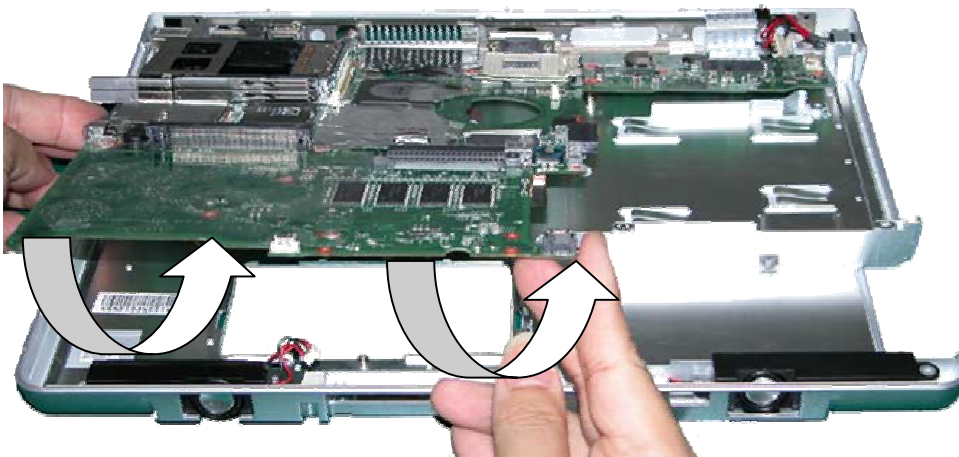
Fig. 33 Lifting up the Main Board
